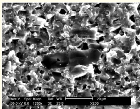
Figure 3: SEM image showing interfacial failure of TSS specimen x1200.
