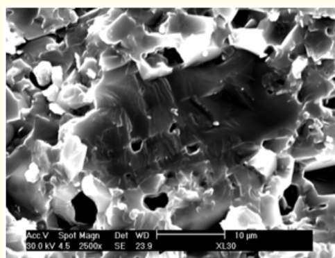
Figure 4: SEM image showing microgaps due to hydrolysis of TSS specimen x2500.
