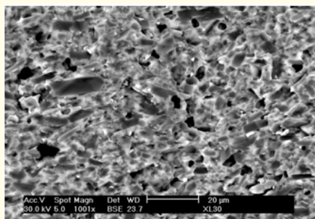
Figure 1: SEM image after SIE of Zirconia x1000.
