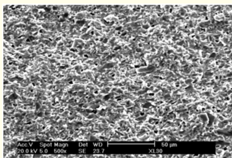
Figure 2: SEM image showing cohesive failure in resin cement x500.
